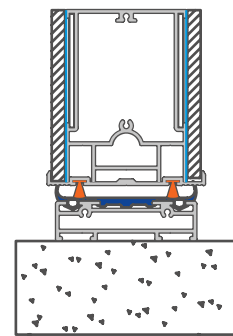
T2 - With Threshold T2 - Με Κατωκάσι T2 - Con Soglia
